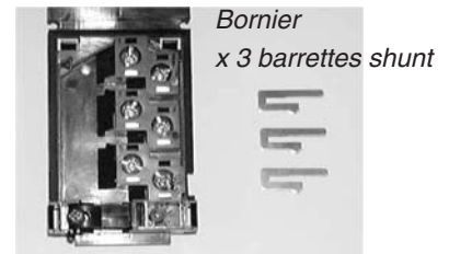
Bornier
