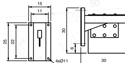
FIXATION STANDARD MURALE
