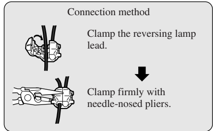
Reversing lamp lead.
