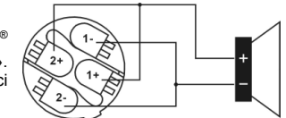
SPEAKON WIRE CONNECTION
