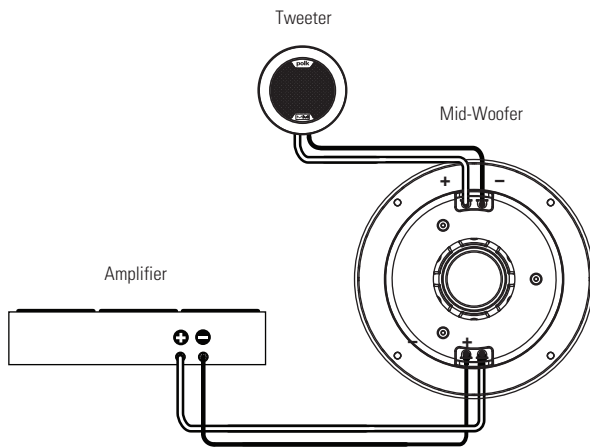
Figure 2 BASIC COMPONENT CONNECTION INSTALLING MM6501UM
