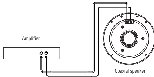
Figure 1 MM651UM BASIC COAXIAL CONNECTION
