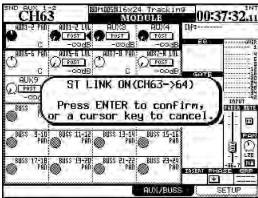
Figure 5.19: Couplage de modules
