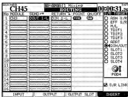
Figure 4.3: Routage des insertions
