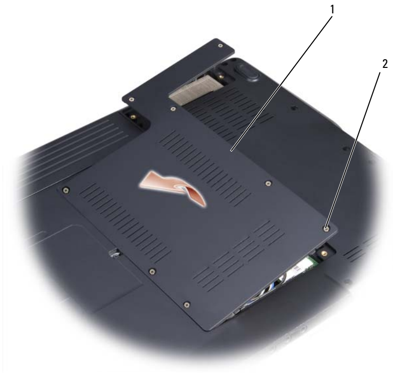
1 capot 2 vis imperdables (5)
