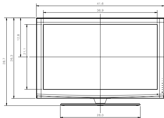
VISTA FRONTAL
