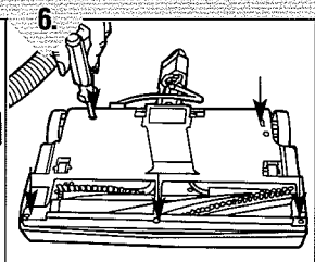
Diagram 6 Replace nozzle guard. Flip power nozzle over and replace the five (5) screws.
