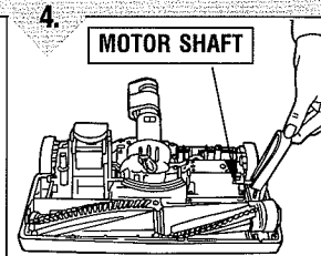
Diagram 4 Pull out broken belt and replace with new belt.
