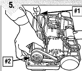
Diagram 5 Insert brushroll into side holder #1 and then #2.
