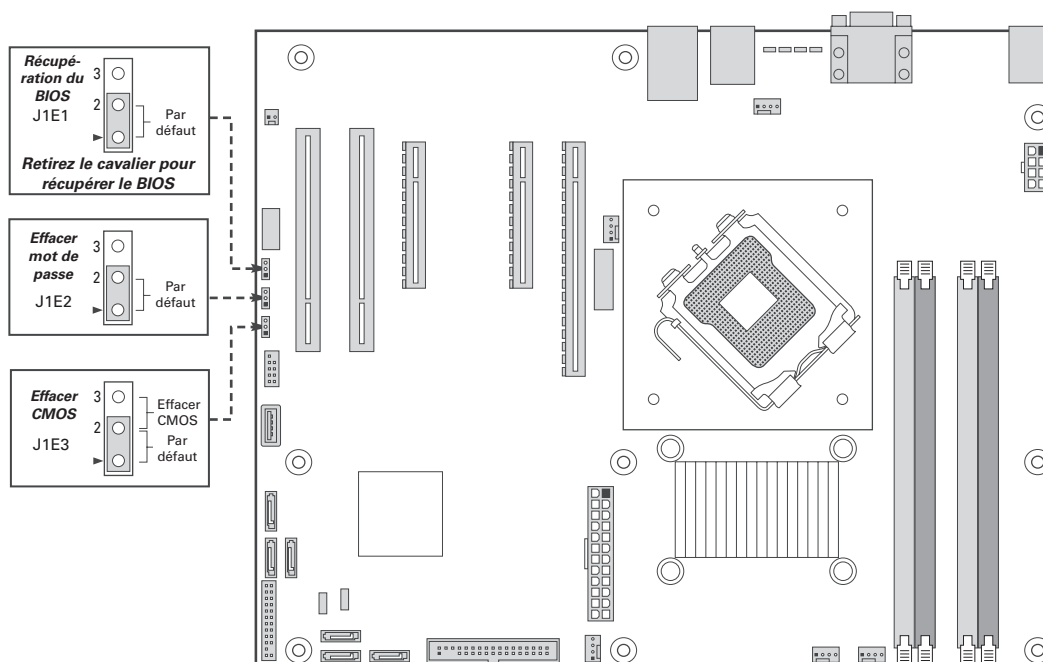
Figure 3. Cavaliers de configuration
