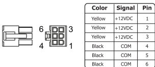
PCI Express Connector (6 Pin)
