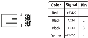
Floppy Disk Connector (4 Pin)
