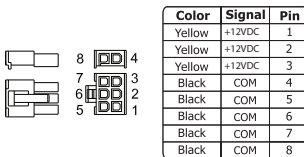
PCI-Express Connector (6+2Pin)
