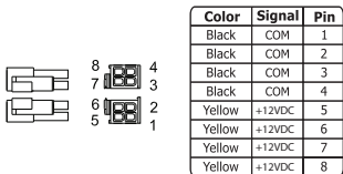
+12V CPU Connector (8 Pin)
