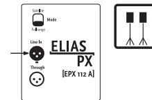
Full-range setup connections
