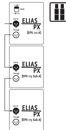
Extension setup connections
