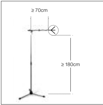
Fig. 3: Antenna mounted on floor stand
