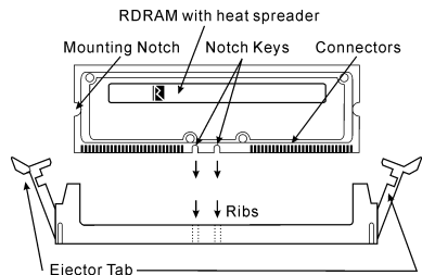
Figure 2-6. Installation des modules mémoire
