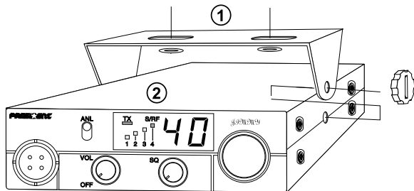
MOUNTING DIAGRAM
