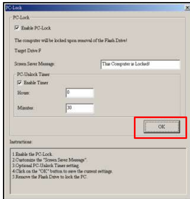
Figure 27: Démarrer PC-Lock
