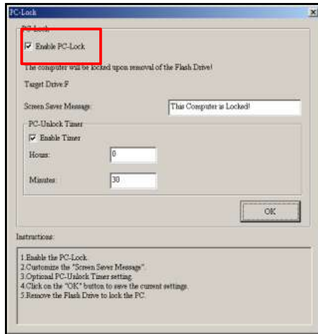
Figure 24: Activer PC-Lock
