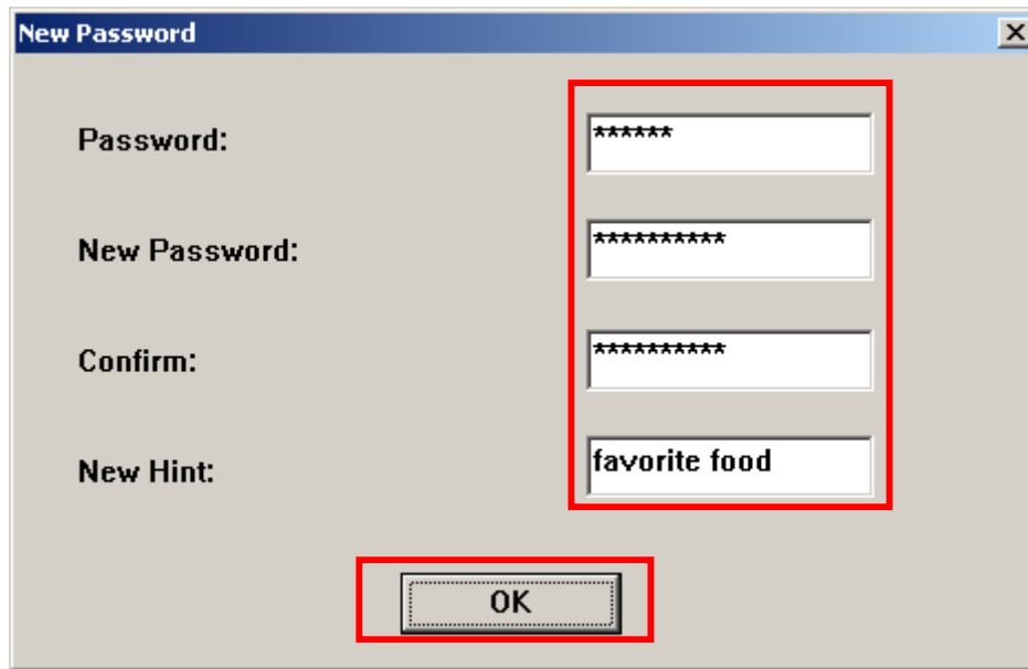
Figure 28. Change Password
