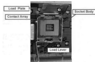
775-Pin Socket Overview
