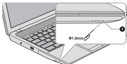
Illustration 4-6 Ejection manuelle
