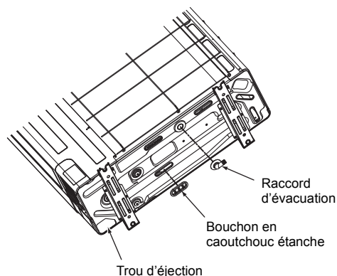
Raccord d'évacuation
