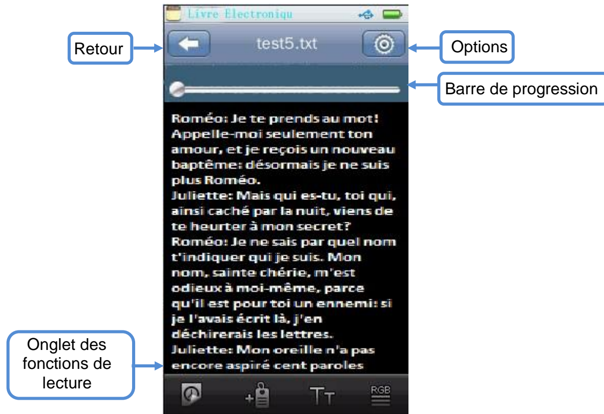
Interface E-Book
