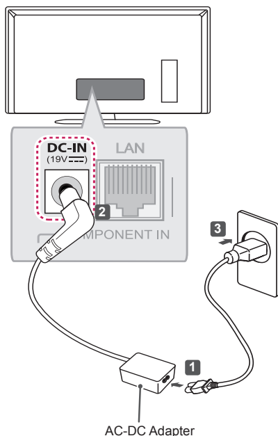
AC-DC Adapter
