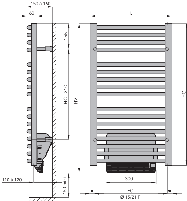
VERSION EAU CHAUDE (...CV)
