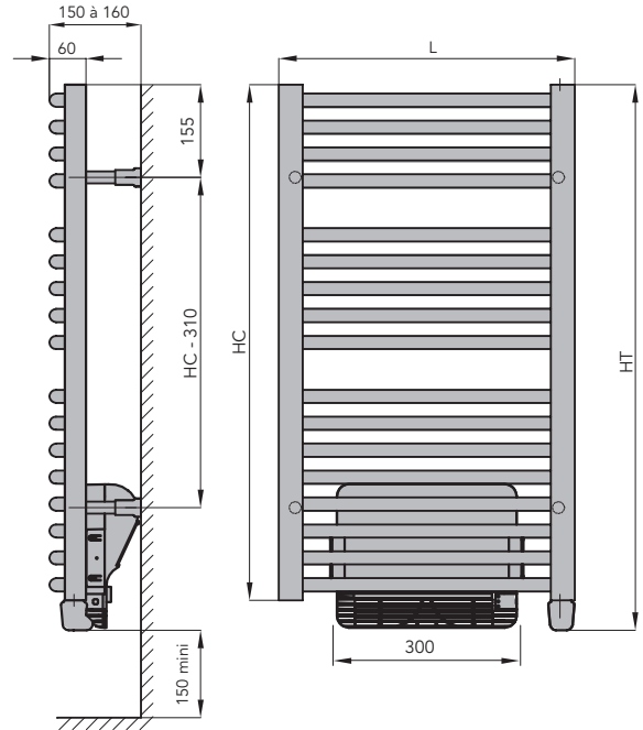
VERSION ELECTRIQUE (...EV)
