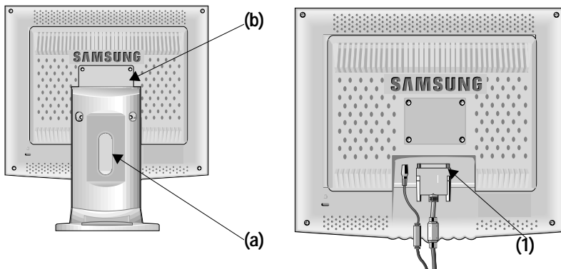
Figure 3.2 Connexion câble DVI-I (uniquement SyncMaster 170T)
