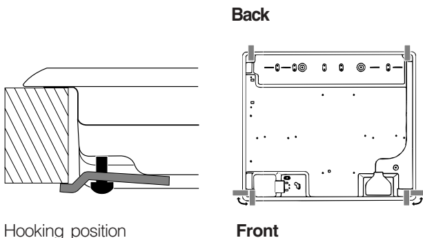
Hooking position for top H=40 mm
