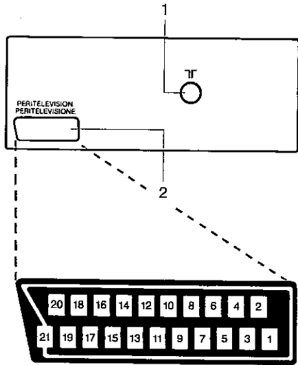
21-pin Euro-SCART
