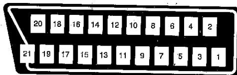
21-polige Euro-SCART-Buchse
