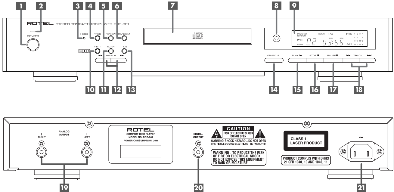
Figure 1: Controls and Connections Commandes et branchements Bedienelemente und Anschlüsse Comandi E Collegamenti Controles y Conexiones Bedieningsorganen en aansluitingen
