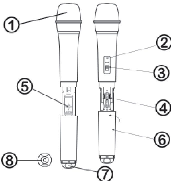
FM-64 MICROPHONE
