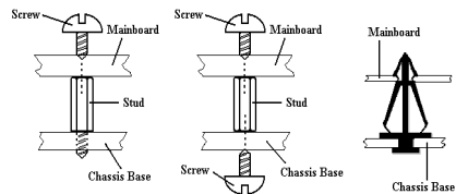
Figure 2-2. The way we fixed the motherboard
