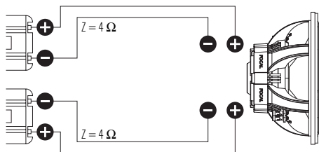
Connection using 2 amplifiers (mono)
