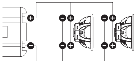
2 subwoofers both in parallel, Z = 1 \Omega
