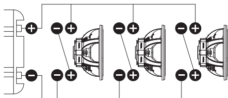
3 subwoofers connected in series / parallel, Z = 2,66 \Omega
