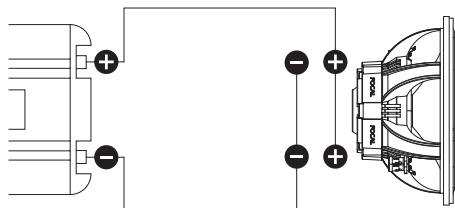
Connect in parallel the 2 voice coils Z = 2 \Omega
