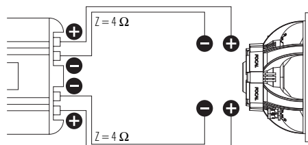
Connection using 1 amplifier (stereo)
