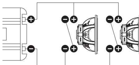
2 subwoofers connected in series / parallel, Z = 4 \Omega
