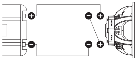
Connect in series the 2 voice coils Z = 8 \Omega
