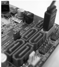
Connect the SATA data cable to the orange SATAII connector (SATAII_6 (PORT5))
