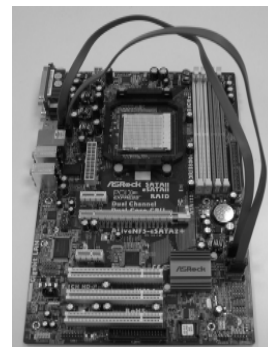
Connect the SATA data cables to both red eSATAII connector (eSATAII_BOTTOM) and orange eSATAII connector (eSATAII_TOP)
