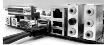
Connect the other end of the eSATAII device cable to eSATAII port of the I/O shield
