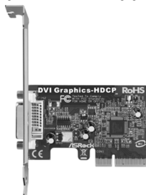
DVI Graphics-HDCP-Karte
