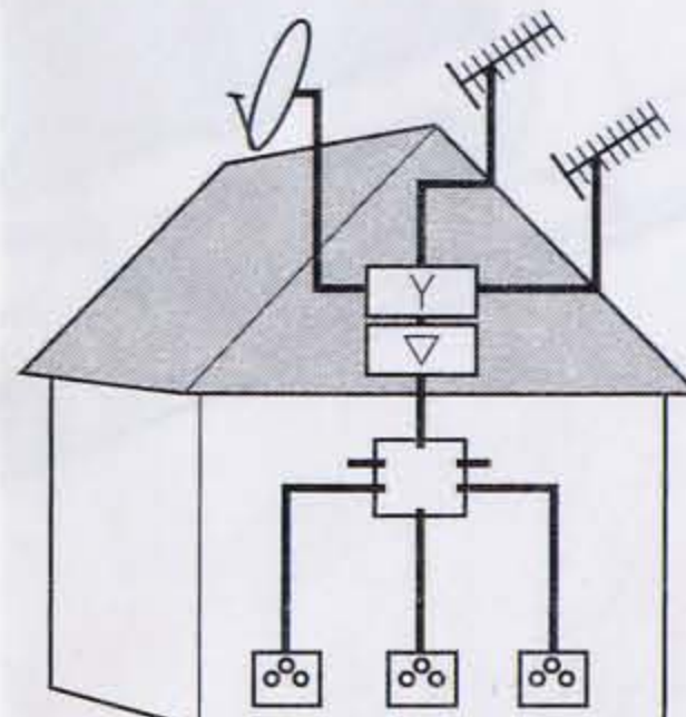
TV - FM SAT hertzian and satellite distribution
