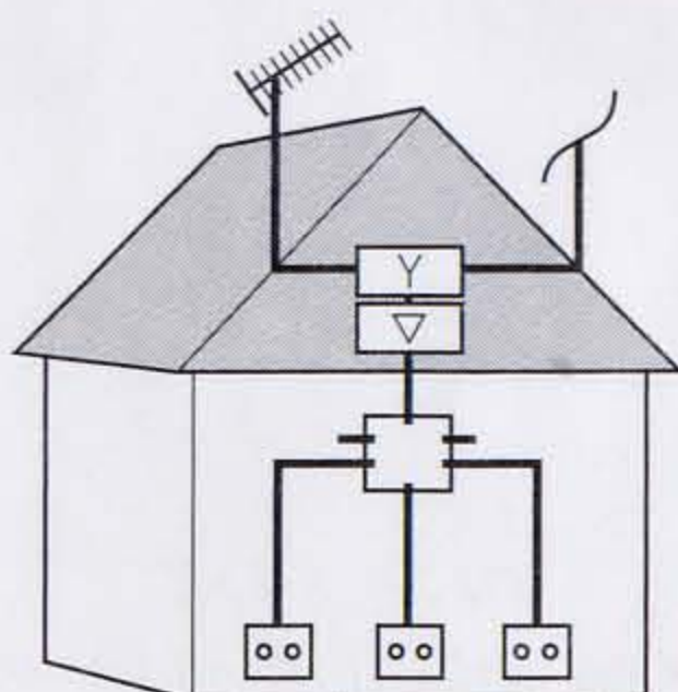
TV - FM hertzian distribution
