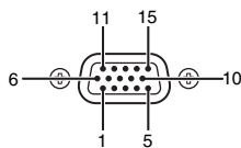
MONITOR IN/OUT (Mini D-SUB 15-broches)
