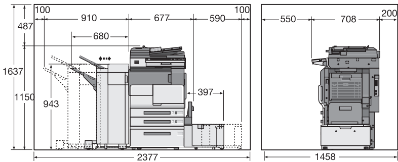
bizhub 500/420 + PC-402 + FS-511 + LU-201
