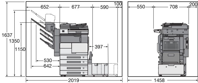
bizhub 500/420 + PC-202 + FS-510 + SD-502 + LU-201
