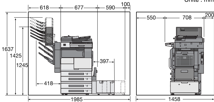
bizhub 500/420 + PC-202 + FS-510 + MT-501 + LU-201
