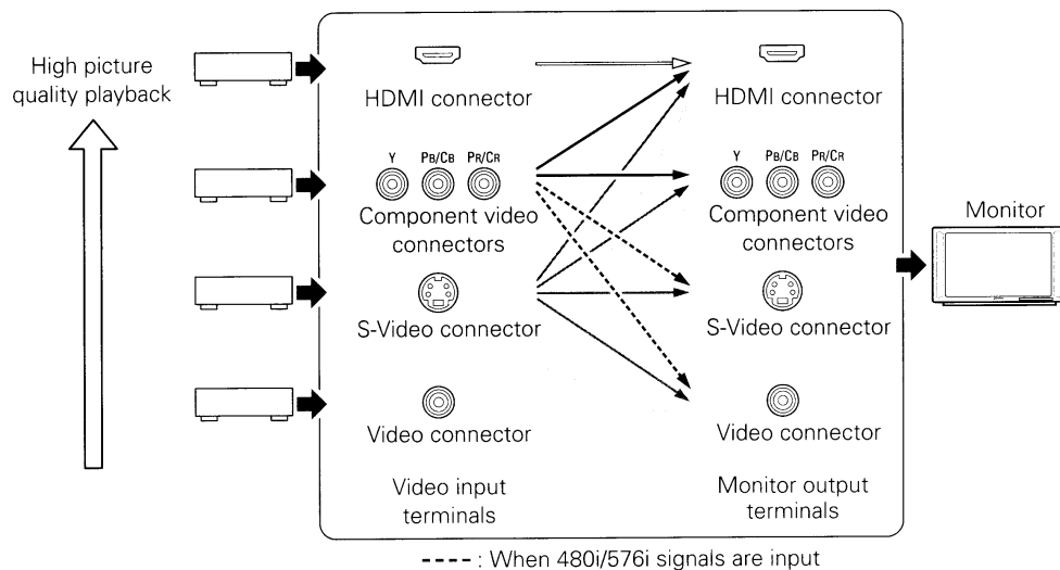
[Flow of video signals inside the AVR-2309CI]
