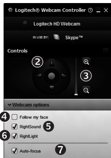
Webcam Controller
