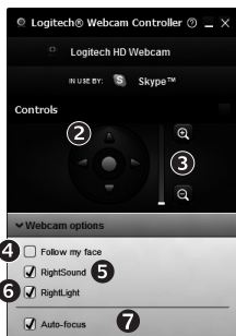
Webcam Controller
