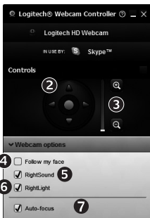
Webcam Controller
