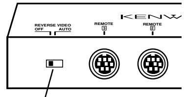
Interruptor selector REVERSE VIDEO AUTO/OFF
