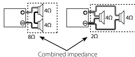
Combined impedance
