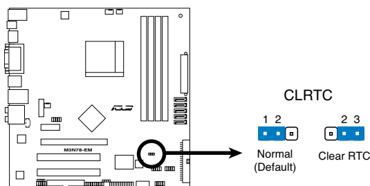
Clear RTC RAM de la M3N78-EM
