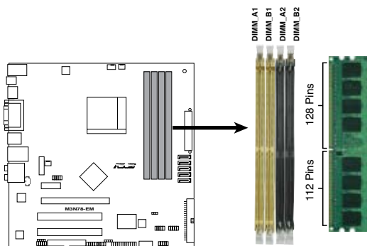
Sockets DIMM DDR2 de la M3N78-EM
