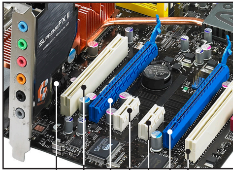
Slot 1 Audio/PCI Express x1
