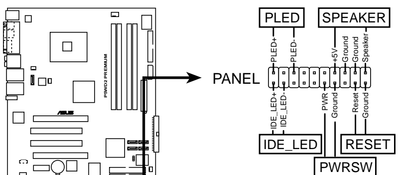
P5WD2 PREMIUM System panel connector
