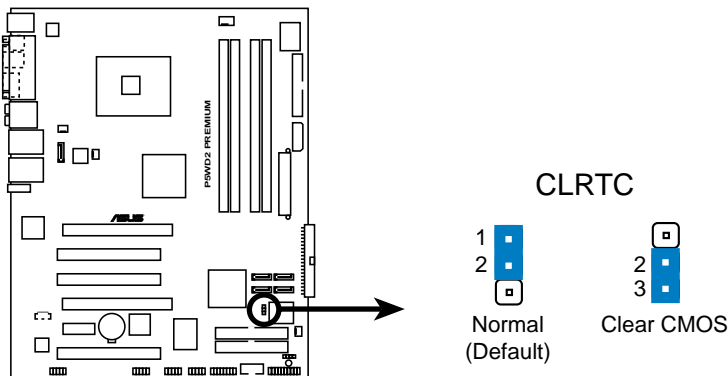
P5WD2 PREMIUM Clear RTC RAM
