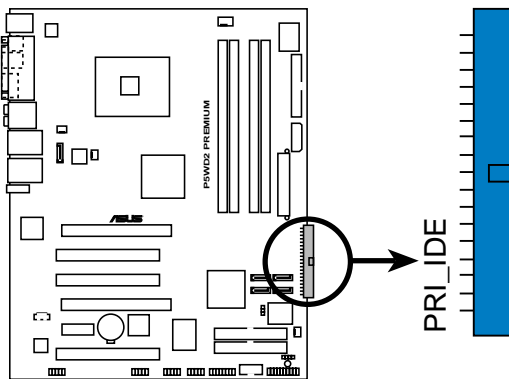
P5WD2 PREMIUM IDE connector
