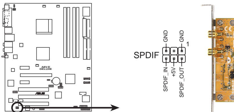
A8V-E DELUXE Digital audio connector
