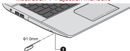
Illustration 4-4 Ejection manuelle
