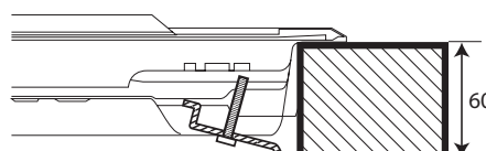
Plan 60 mm
