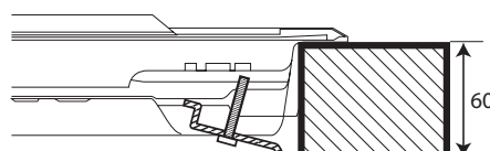
Plan 60 mm
