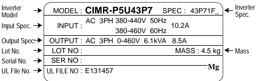
Figure 1 Nameplate Example of American Model CIMR-P5U43P7
