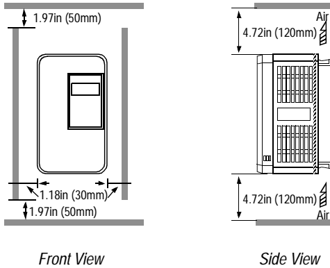
Figure 8 VS-616PC5/P5 Clearances
