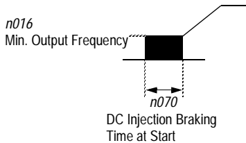
Figure 45 DC Injection Braking at Starting
