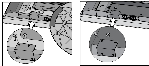
Main switch cover (with stand) The longer side of the cover is toward the bottom of the display.
